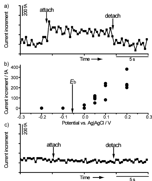
Figure 2. a) Representative current response from a single bacterial cell. An optically trapped microbe was attached and detached from the ITO electrode by using optical tweezers. Prior to the measurements, the microbe was cultured at +200 mV for 1 day. The electrode potential was set at +200 mV. b) Current responses of a single microbe by using electrodes poised at various potentials. Microbes cultured at +200 mV for 1 day were used for the analyses. The arrow indicates the potential ( E_b ) at which the relative amounts of oxidized and reduced forms of OMC were balanced under the operation conditions. [2a] c) Representative current response for a single cell precultured at −200 mV. The experiment was performed similarly to that described in (a).
