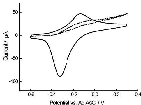
Figure 3. Whole-cell cyclic voltammograms of a microbial suspension cultured electrochemically at either +200 mV (—) or –200 mV (----) for 1 day prior to the measurement. Microbial cell suspensions with an optical cell density at 600 nm of 2.0 were used. The scan rate of the potential was 50 mV s -1 .
